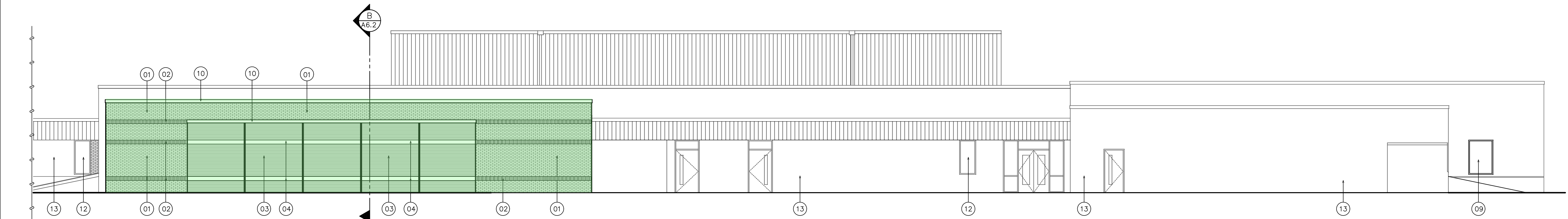
03 PARTIAL NORTH ELEVATION SCALE: 1/8" = 1'-0"
