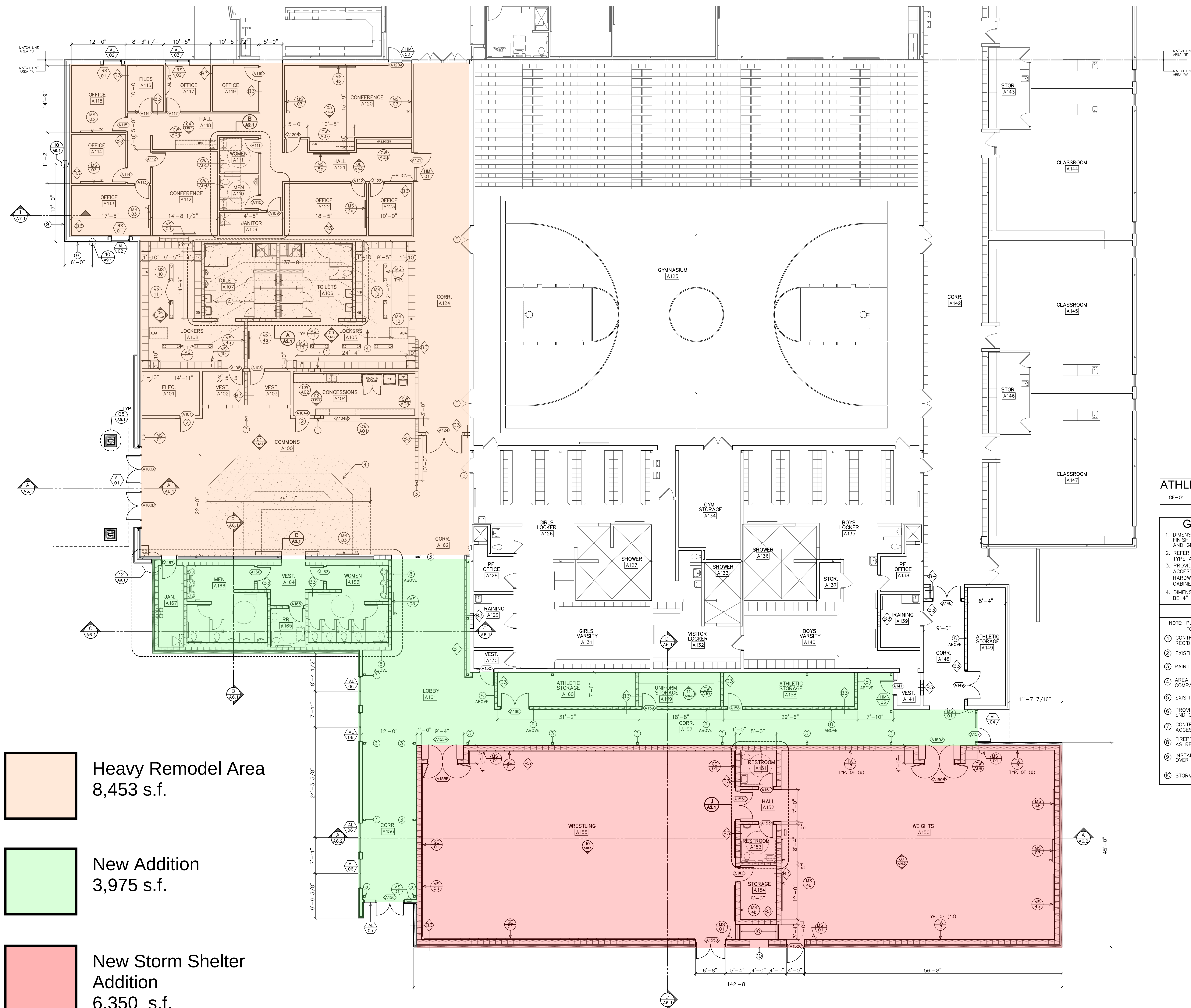
AREA 'A' FLOOR PLAN SCALE: 1/8" = 1'-0"
