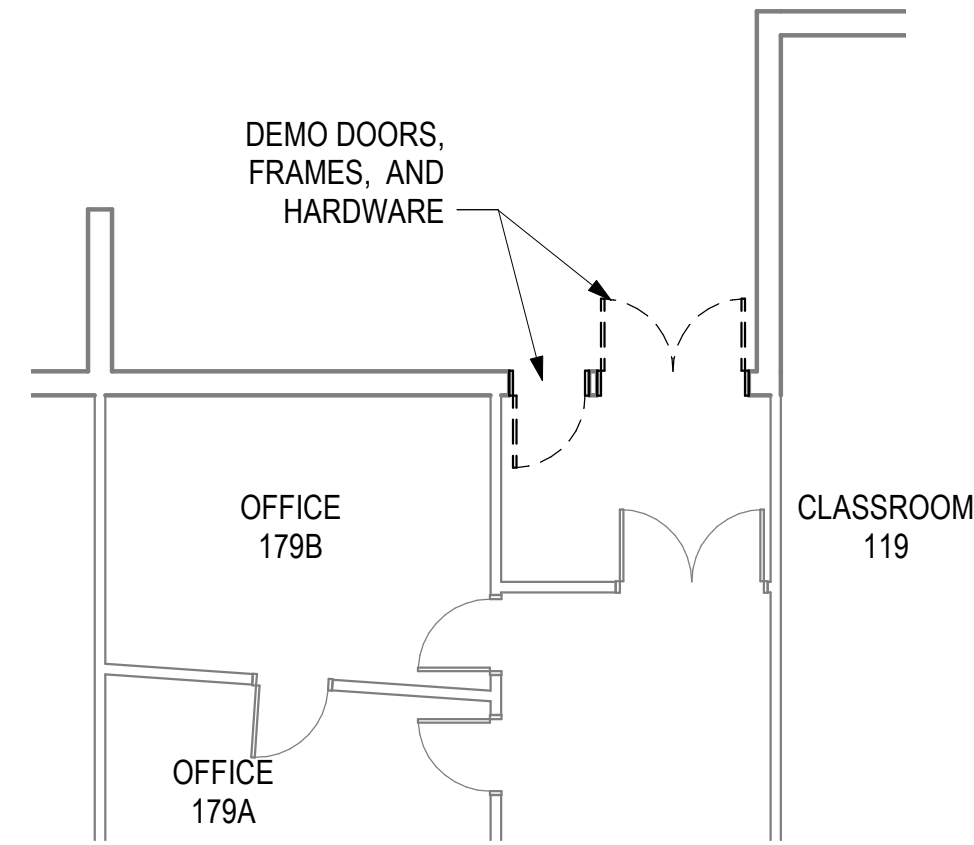
1 A111 NOME-BELTZ BUS ACCESS - DEMO 1/8" = 1'-0"
