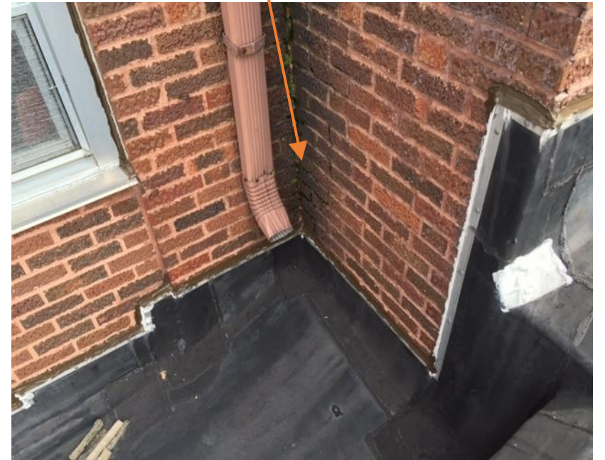
Gutter Damage
