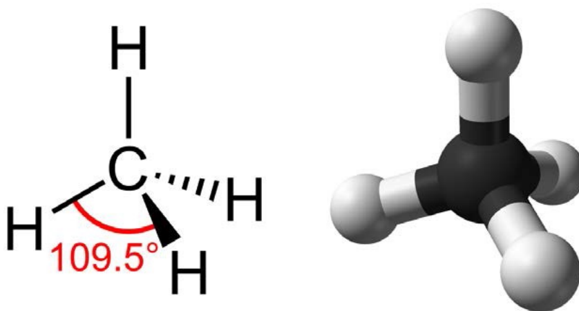
Figure 1.2. Methane ( \text{CH}_4 ) has a tetrahedral geometry, with each of the four hydrogen atoms spaced 109.5^\circ apart.
