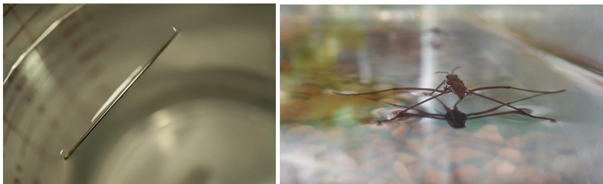
Figure 8.5 The weights of the needle and water strider are pulling the surface downward; at the same time, the surface tension is pulling it up, suspending them on the surface of the water and keeping them from sinking. (Credit: Cory Zanker (left) and Tim Vickers (right))
