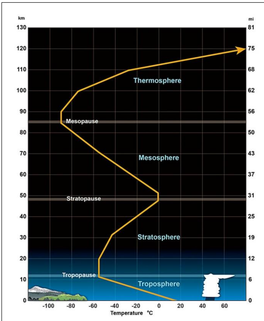
Figure 6.1: An average temperature profile through the lower layers of the atmosphere. Height (in miles and kilometers) is indicated along each side. Source: National Weather Service
