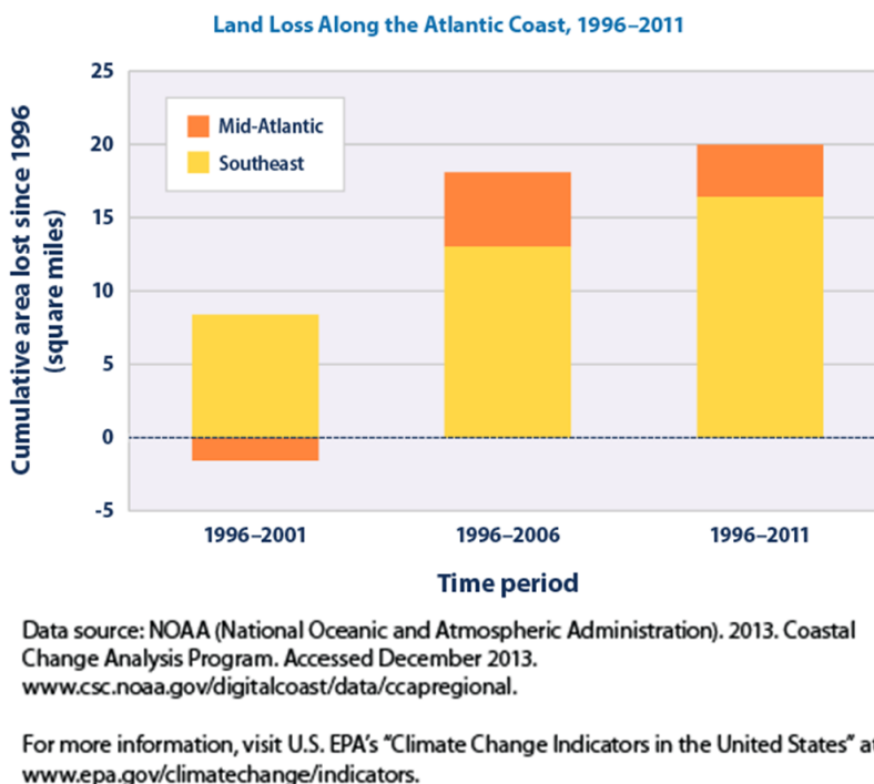
Figure 7.17. This graph shows the net amount of land converted to open water along the Atlantic coast during three time periods: 1996–2001, 1996–2006, and 1996–2011. The results are divided into two regions: the Southeast and the Mid-Atlantic. Negative numbers show where land loss is outpaced by the accumulation of new land.
