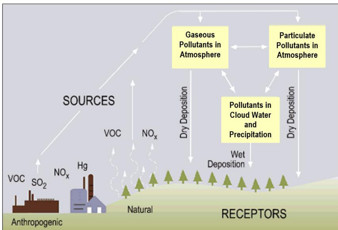
Figure 6.12: Formation of acid rain from both natural and anthropogenic pollutants
