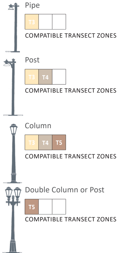
FIGURE 4-4: STREET LIGHTING
