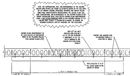
ANGLE FRAMING DETAIL S1.0-5
