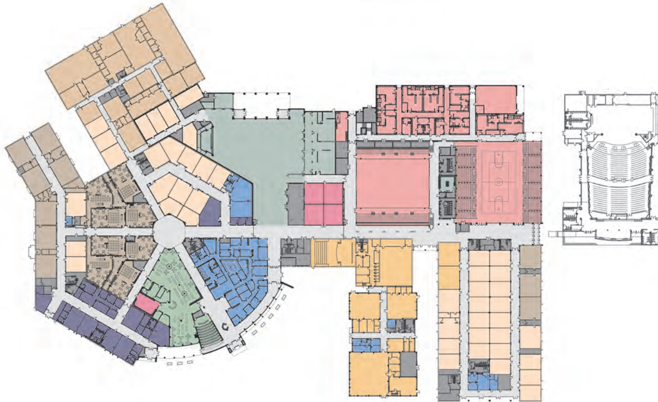
Master Floor Plan
