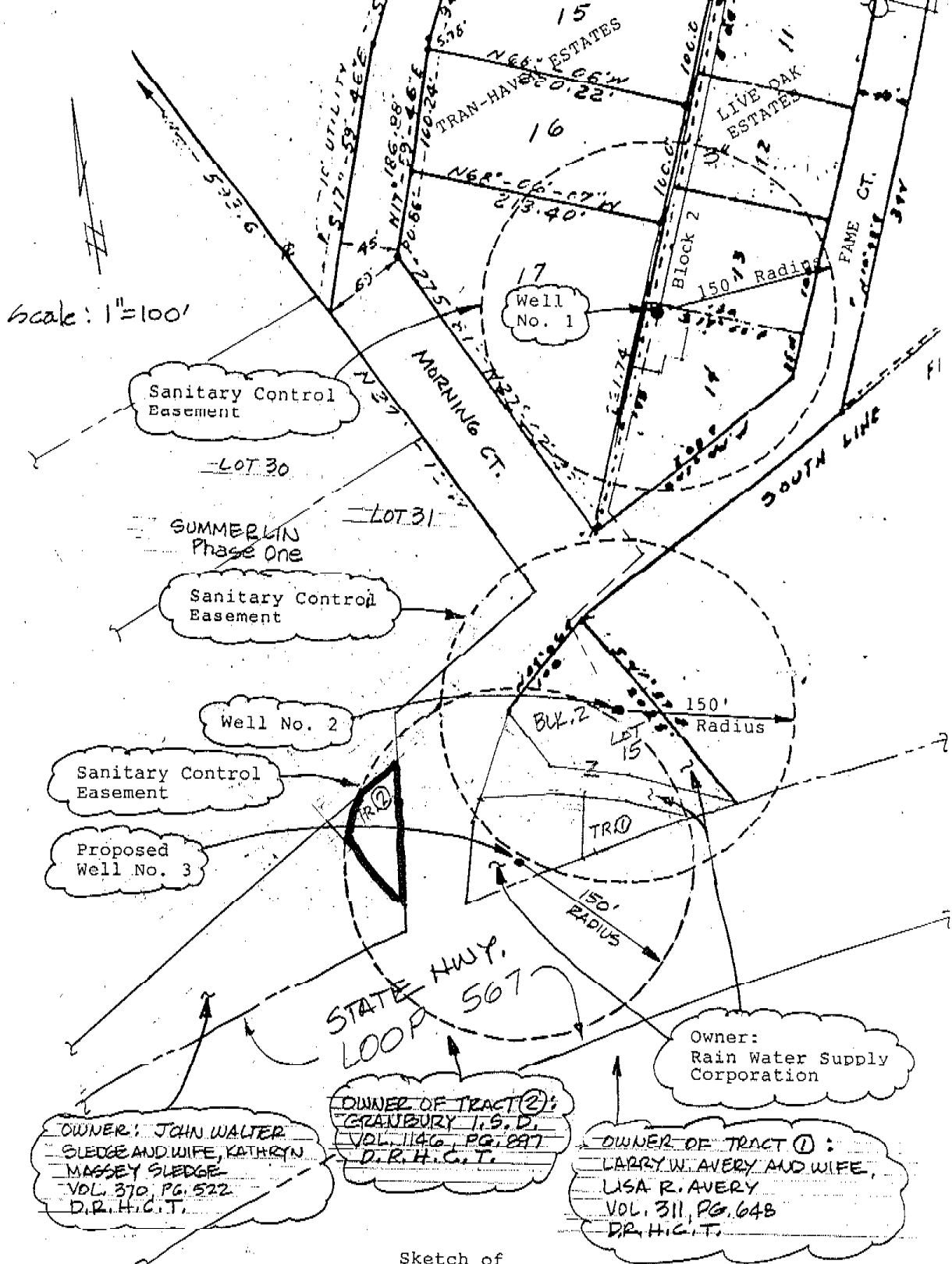
Sketch of SANITARY CONTROL EASEMENTS Wells No. 1, 2 & 3
