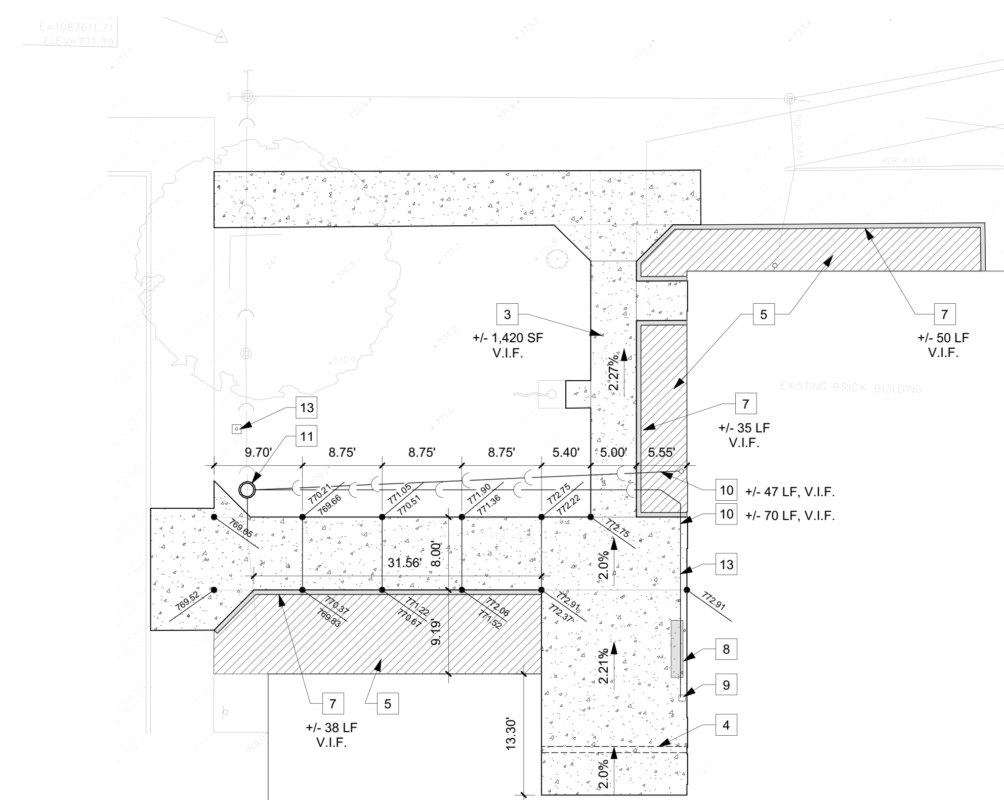
4 PARTIAL SITE PLAN - NORTH 3/32" = 1'-0"
