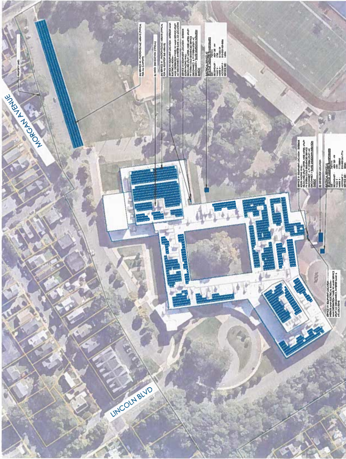
SITE PLAN SCALE: 1" = 80'
