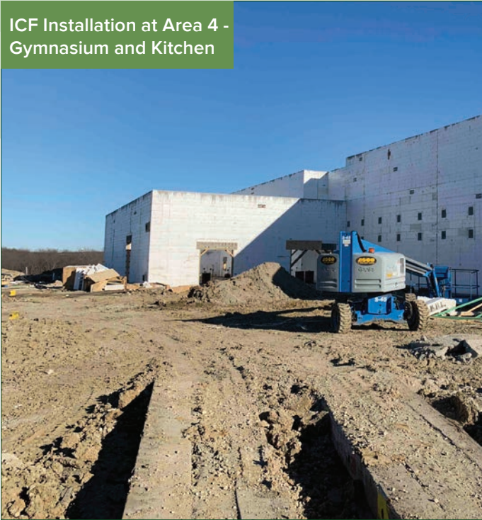
ICF Installation at Area 4 - Gymnasium
