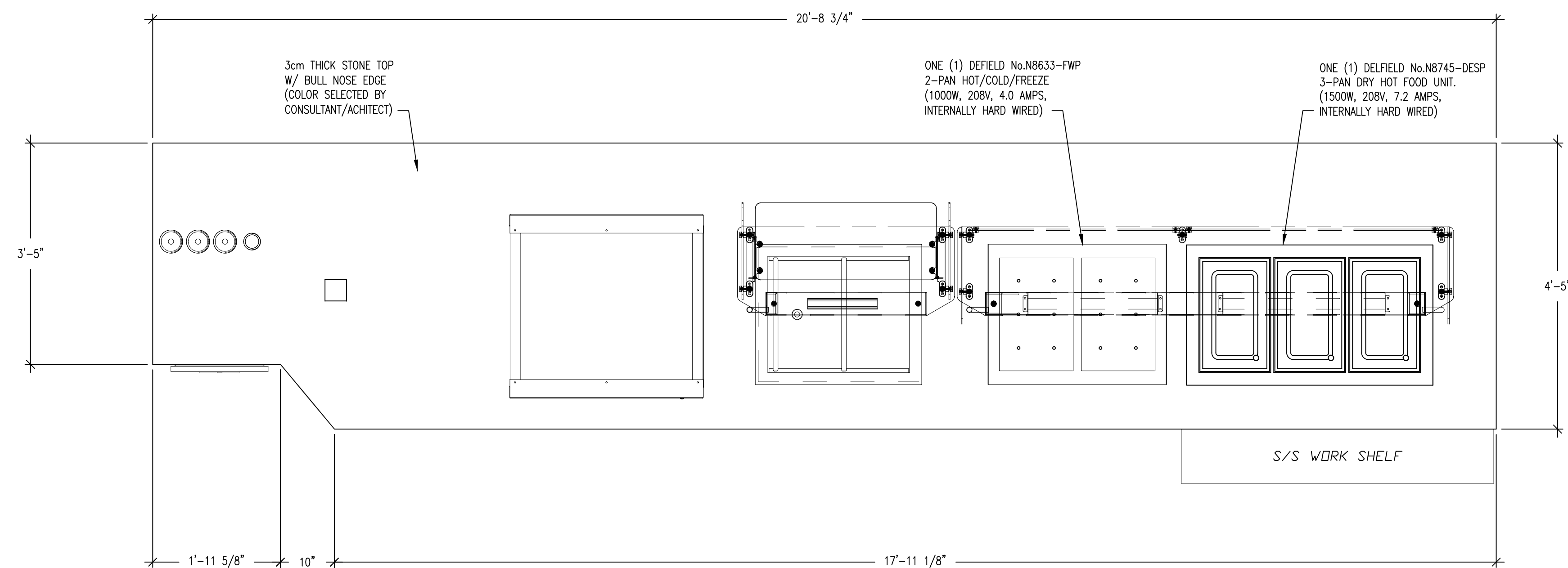
PLAN OF THE ROCK SERVING COUNTER ITEM No.105 ONE (1) REQ'D SCALE: 3/4"=1'-0"
