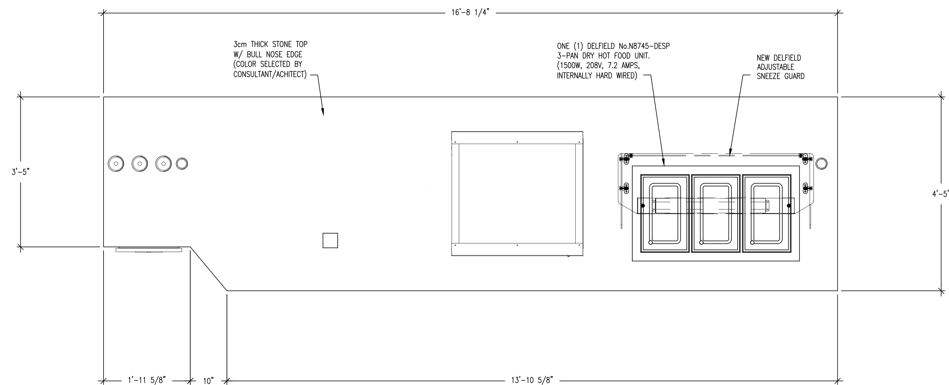
PLAN OF THE JACKET GRILL SERVING COUNTER ITEM No.103 ONE (1) REQ'D SCALE: 3/4"=1'-0"
