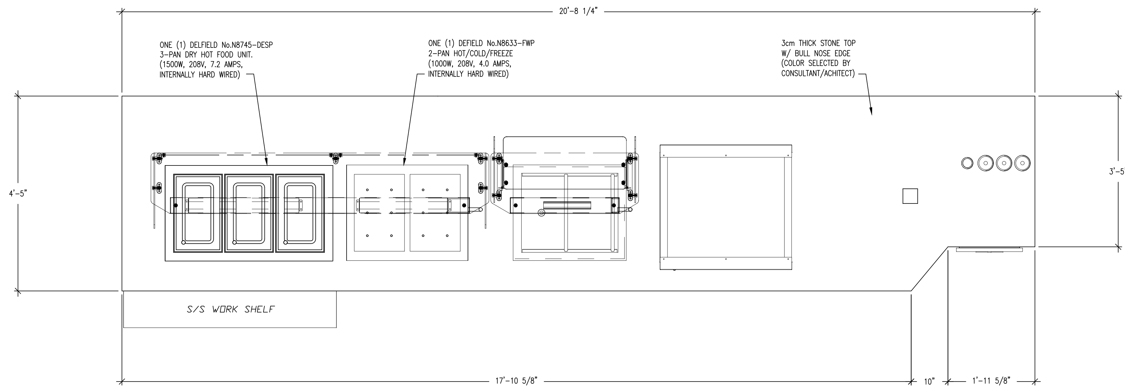
PLAN OF MEXICAN TACO SHED SERVING COUNTER ITEM No.102 ONE (1) REQ'D SCALE: 3/4"=1'-0"
