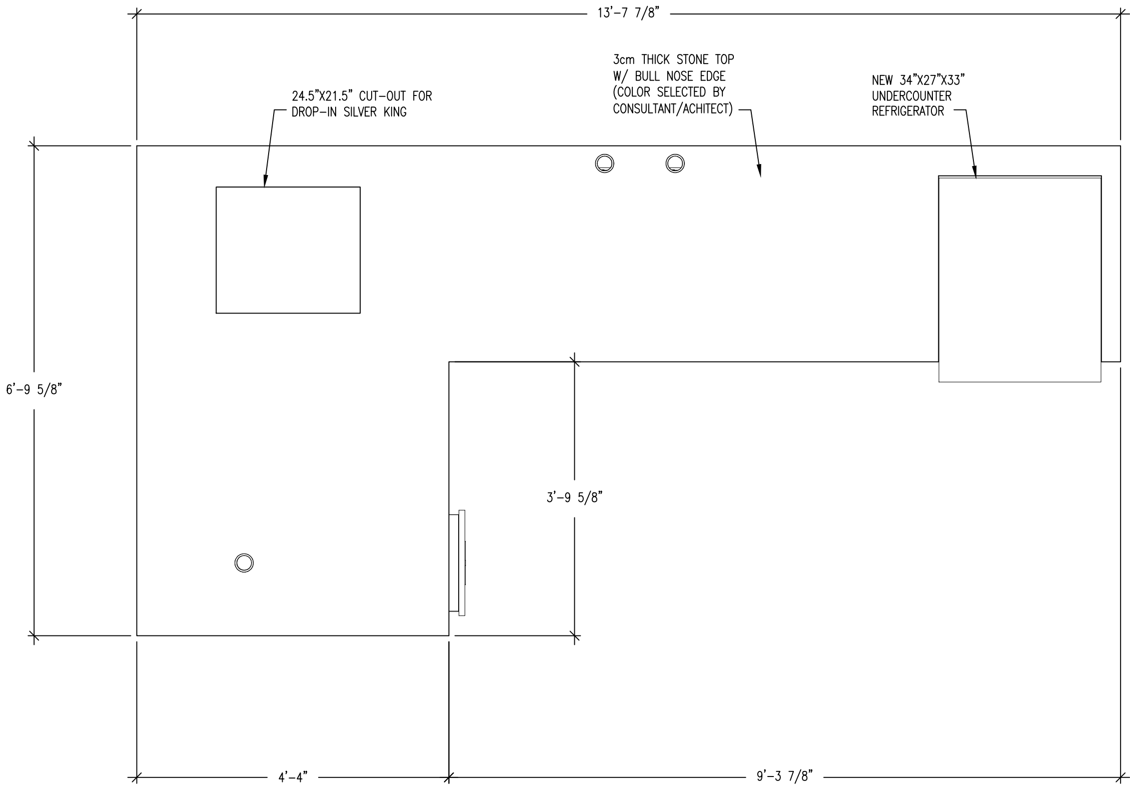
PLAN OF DELI DEPOT CASHIER SERVING COUNTER
