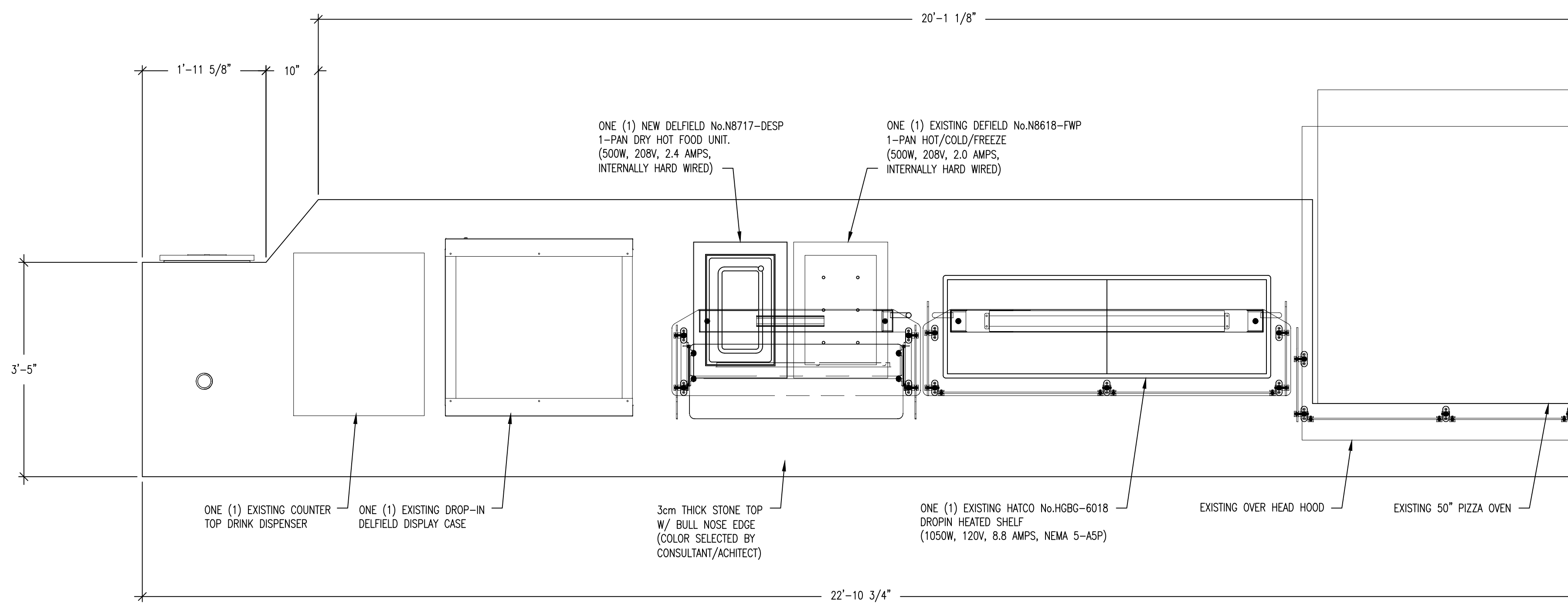
PLAN OF PIZZA SERVING COUNTER ITEM No.106 ONE (1) REQ'D SCALE: 3/4"=1'-0"
