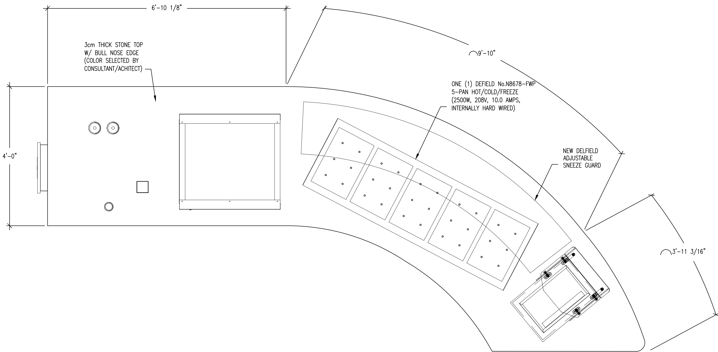
PLAN OF DELI SERVING COUNTER ITEM No.101 ONE (1) REQ'D SCALE: 3/4"=1'-0"
