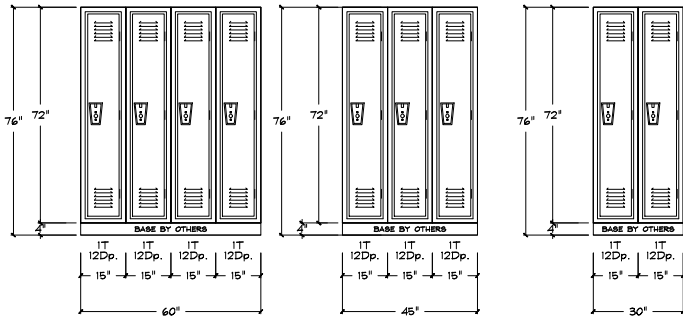
1 LOCKER RUNS A-C 15X12X72 C1 SCALE: 3/8" = 1'-0" ARCHITECTURAL REF. LOCKER EXTERIOR: ADVISE COLOR LOCKER TYPE: REPUBLIC STANDARD IT KD LOCKER LOCKERTOPS: FLAT TOPS LOCKS: BY OTHERS BASE: BY OTHERS
