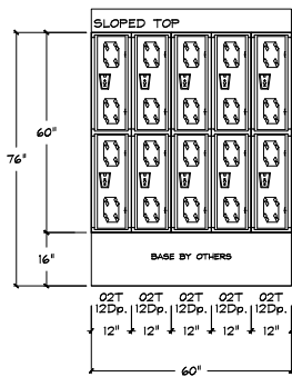
5 LOCKER ROOMS 456 & 471 M-O C3 SCALE: 3/8" = 1'-0" ARCHITECTURAL REF.
