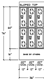
5 LOCKER ROOMS 456 & 471 M-O C3 SCALE: 3/8" = 1'-0" ARCHITECTURAL REF.
