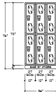
4 WRESTLING LOCKERS RUNS K-L SCALE: 3/8" = 1'-0" ARCHITECTURAL REF. LOCKER EXTERIOR: ADVISE COLOR LOCKER TYPE: DEBOURGH WELDED ANGLE IRON 2T LOCKERTOPS: FLAT TOPS LOCKS: BY OTHERS BASE: BY OTHERS
