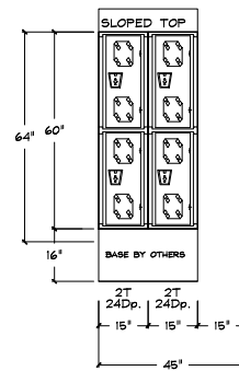
6 LOCKER ROOMS 456 & 471 P-R C3 SCALE: 3/8" = 1'-0" ARCHITECTURAL REF.
