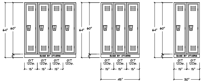
2 LOCKER RUNS D-F 15X12X60 C1 SCALE: 3/8" = 1'-0" ARCHITECTURAL REF. LOCKER EXTERIOR: ADVISE COLOR LOCKER TYPE: REPUBLIC STANDARD IT KD LOCKER LOCKERTOPS: FLAT TOPS LOCKS: BY OTHERS BASE: BY OTHERS
