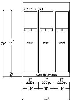
3 FOOTBALL LOCKERS RUNS G-I SCALE: 3/8" = 1'-0" ARCHITECTURAL REF. LOCKER EXTERIOR: ADVISE COLOR LOCKER TYPE: DEBOURGH WELDED ANGLE IRON/NO DOORS LOCKERTOPS: SLOPED TOP LOCKS: BY OTHERS BASE: BY OTHERS
