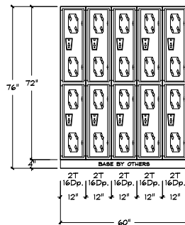
4 WRESTLING LOCKERS RUNS K-L SCALE: 3/8" = 1'-0" ARCHITECTURAL REF. LOCKER EXTERIOR: ADVISE COLOR LOCKER TYPE: DEBOURGH WELDED ANGLE IRON 2T LOCKERTOPS: FLAT TOPS LOCKS: BY OTHERS BASE: BY OTHERS
