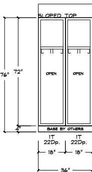
3 FOOTBALL LOCKERS RUNS G-I SCALE: 3/8" = 1'-0" ARCHITECTURAL REF. LOCKER EXTERIOR: ADVISE COLOR LOCKER TYPE: DEBOURGH WELDED ANGLE IRON/NO DOORS LOCKERTOPS: SLOPED TOP LOCKS: BY OTHERS BASE: BY OTHERS
