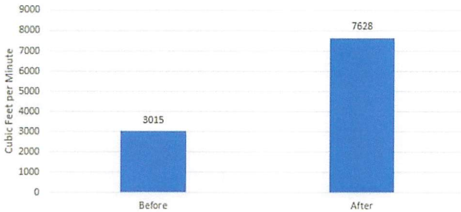
Average Air Flow Readings - Bottom Half SC-3
