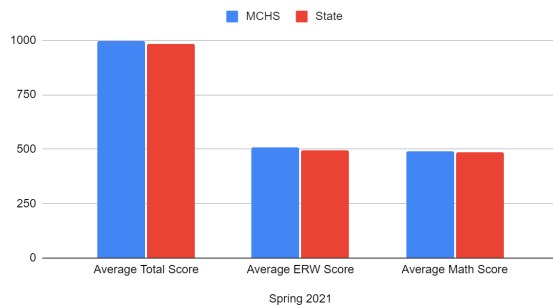
Average Scores
