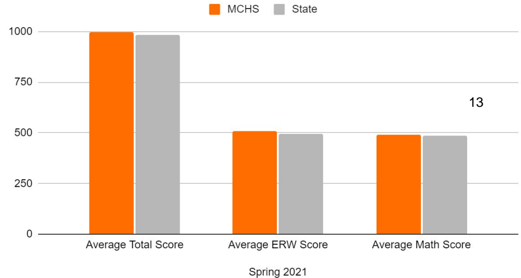
Average Scores
