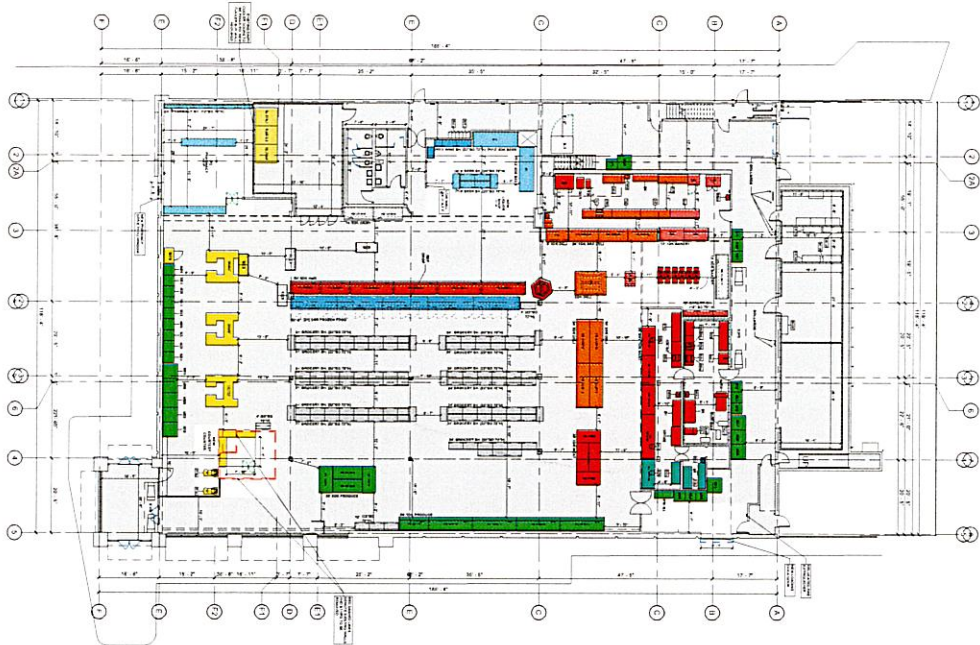
1 MAIN FLOOR 1/16" = 1'-0"
