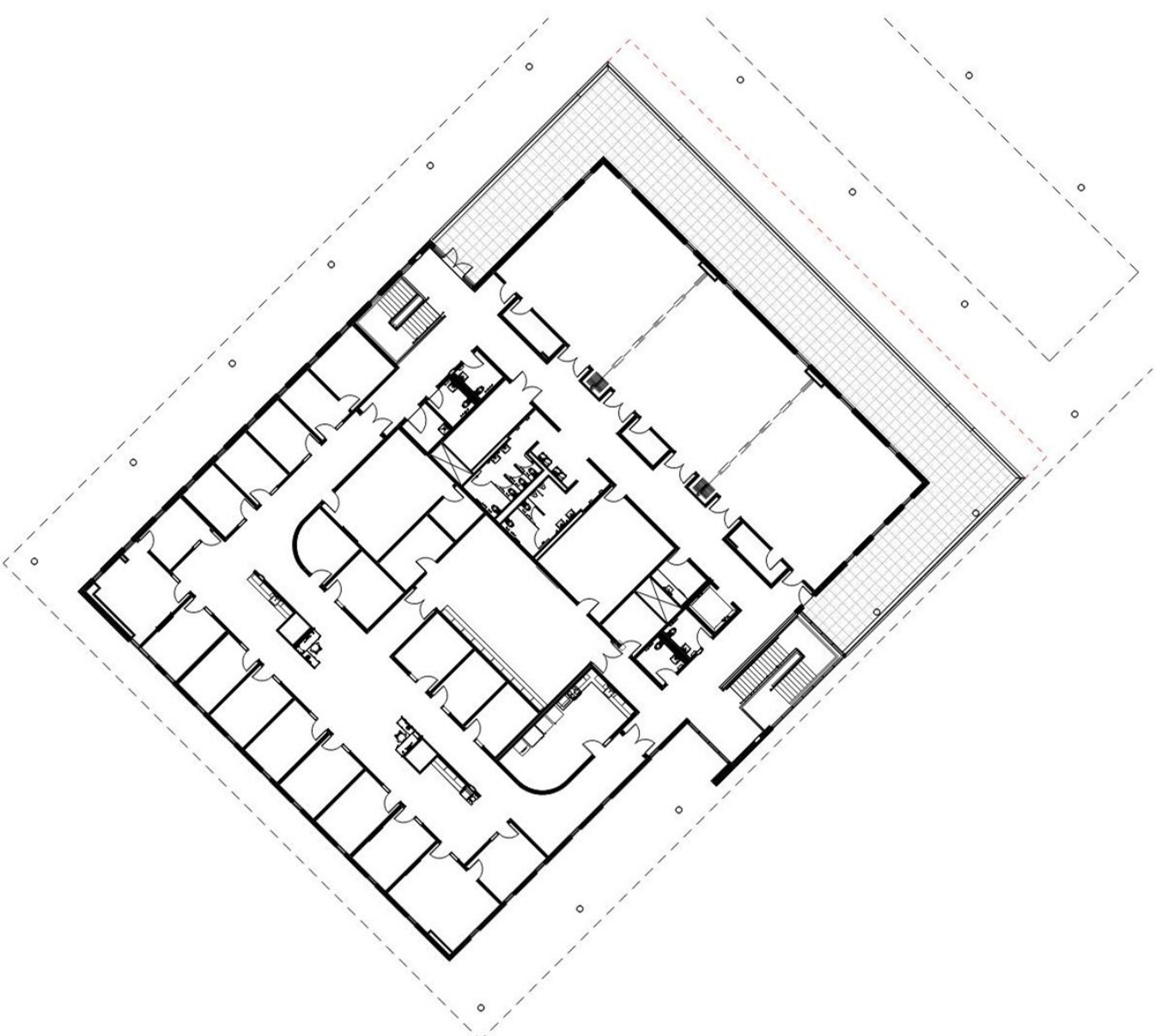
level 02 floor plan - reduced
