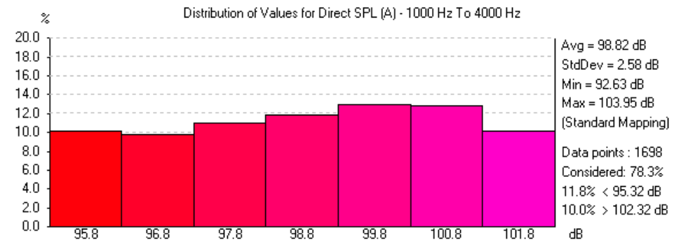
(c) EASE 4.4 / Dover Eyota School Gym / 1/30/2024 4:09:15 PM / Sim Sound and Video, Inc Ian j Sim
