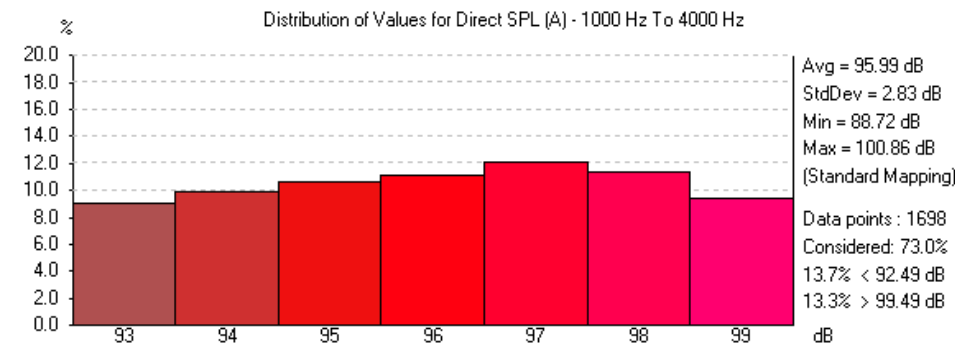
(c) EASE 4.4 / Dover Eyota School Gym / 1/30/2024 4:03:49 PM / Sim Sound and Video, Inc Ian j Sim
