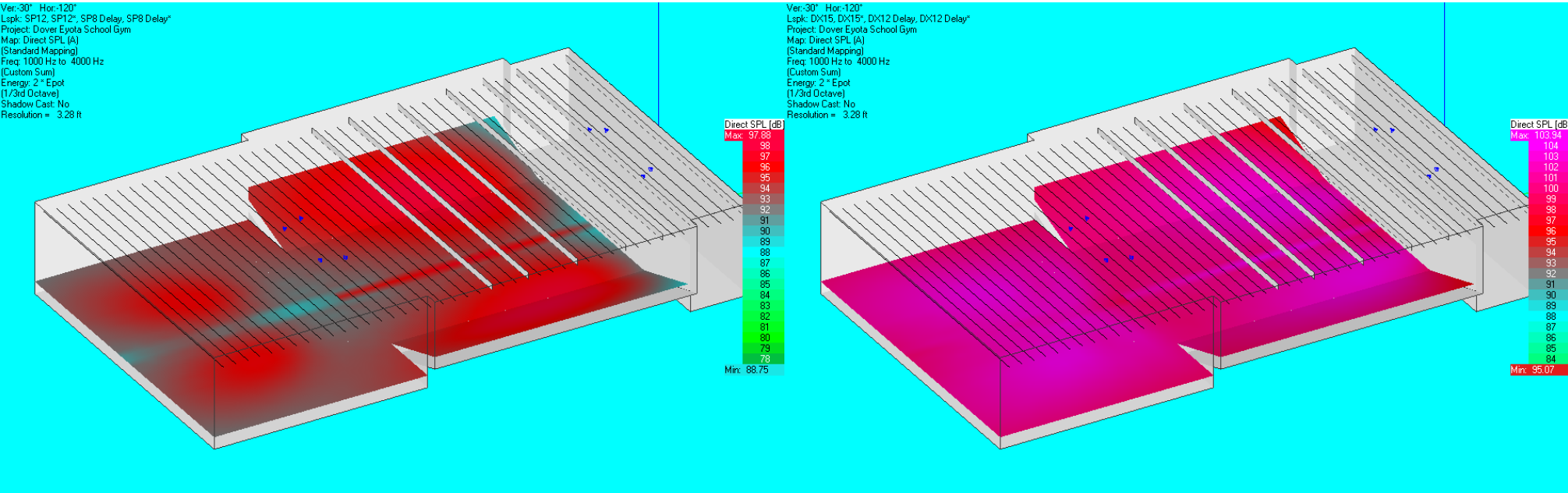
Front Coverage 2 One System SP12D and 2 One System 118HSB Loudspeakers Shown. Back Coverage 2 One System SP8 Loudspeakers Shown.
