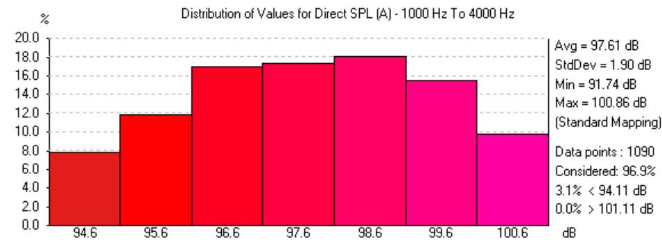
(c) EASE 4.4 / Dover Eyota School Gym / 1/30/2024 3:59:37 PM / Sim Sound and Video, Inc Ian j Sim
