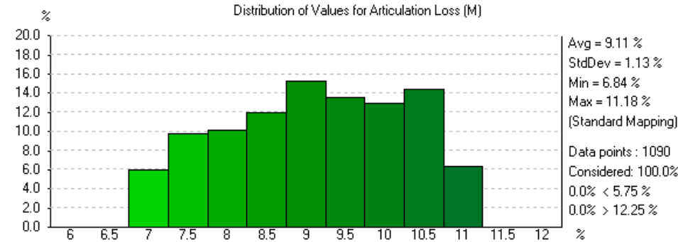
(c) EASE 4.4 / Dover Eyota School Gym / 1/30/2024 4:12:08 PM / Sim Sound and Video, Inc Ian j Sim
