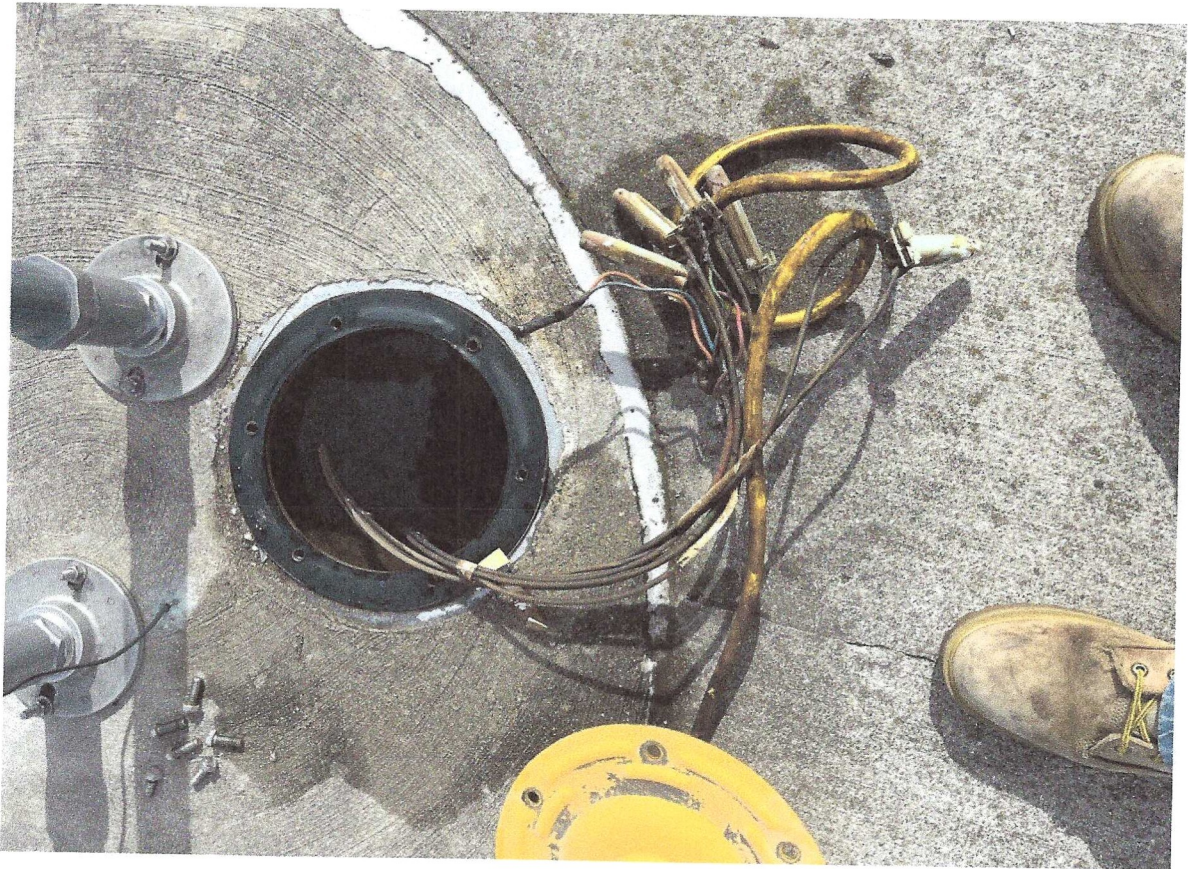
May 5, 2026 PAPI lights Runway 9- underground electric box - full of water
