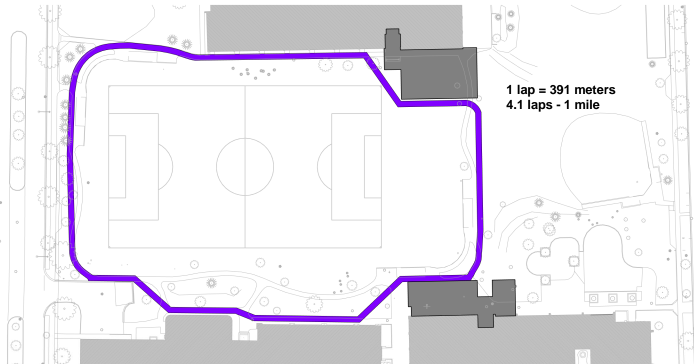
② Running Track - option 2A 1" = 100'-0"
