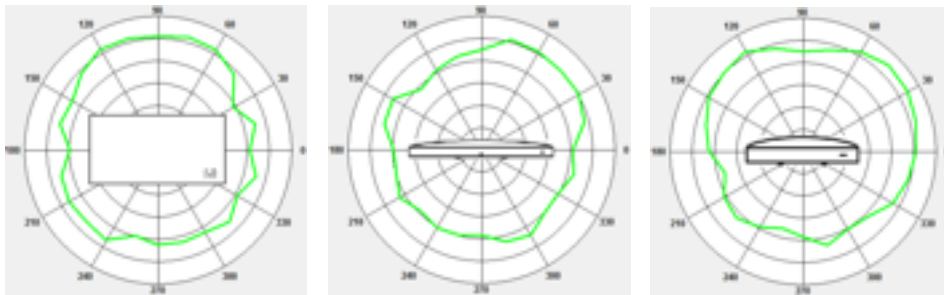
Radiation Pattern for 5GHz Antenna
