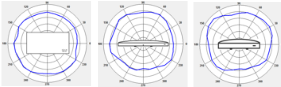
Radiation Pattern for 2.4GHz Antenna
