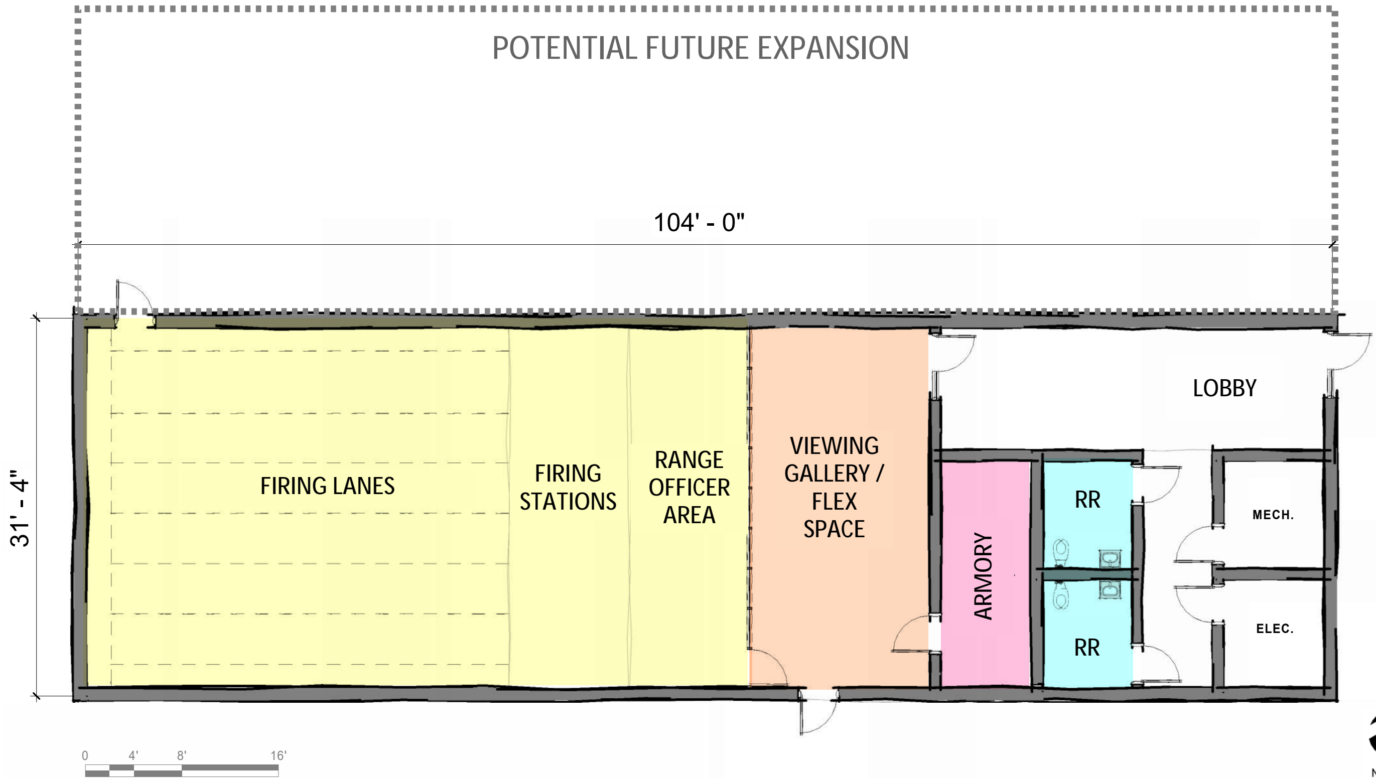
FLOOR PLAN - "MUST HAVE"
