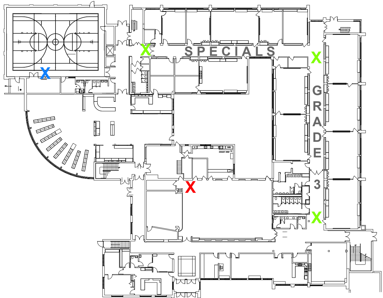
RUTLEDGE HALL FIRST FLOOR PLAN
