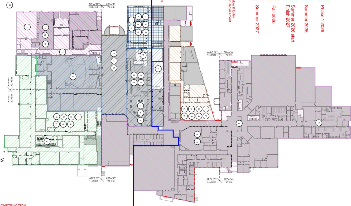
1. OVERALL FIRST FLOOR EXISTING/ DEMOLITION PLAN AD100 1" = 32'-0"
