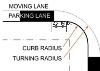
FIGURE 4-2: CURB RADIUS
