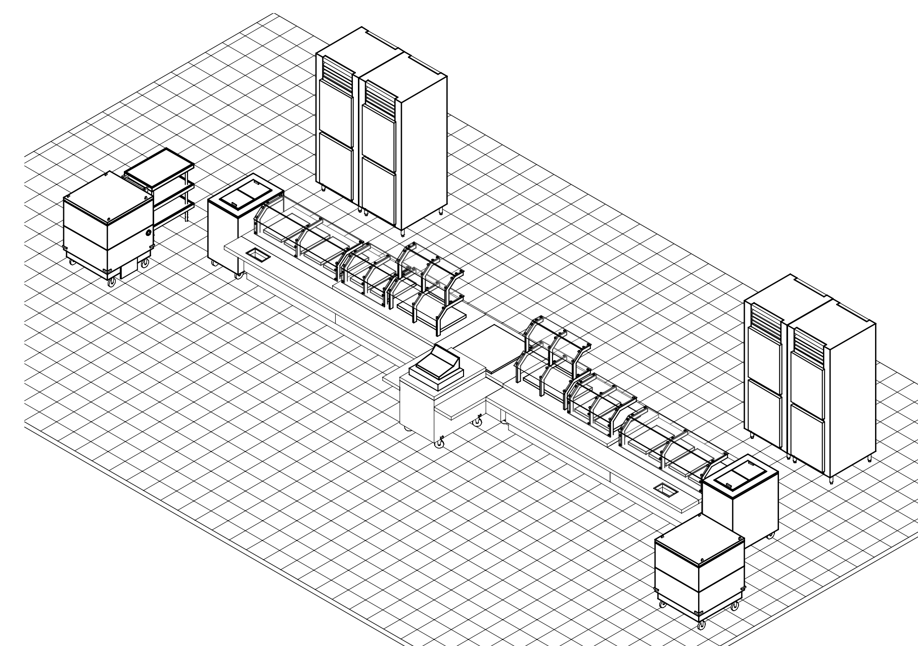
2 FS EQUIPMENT ONLY
