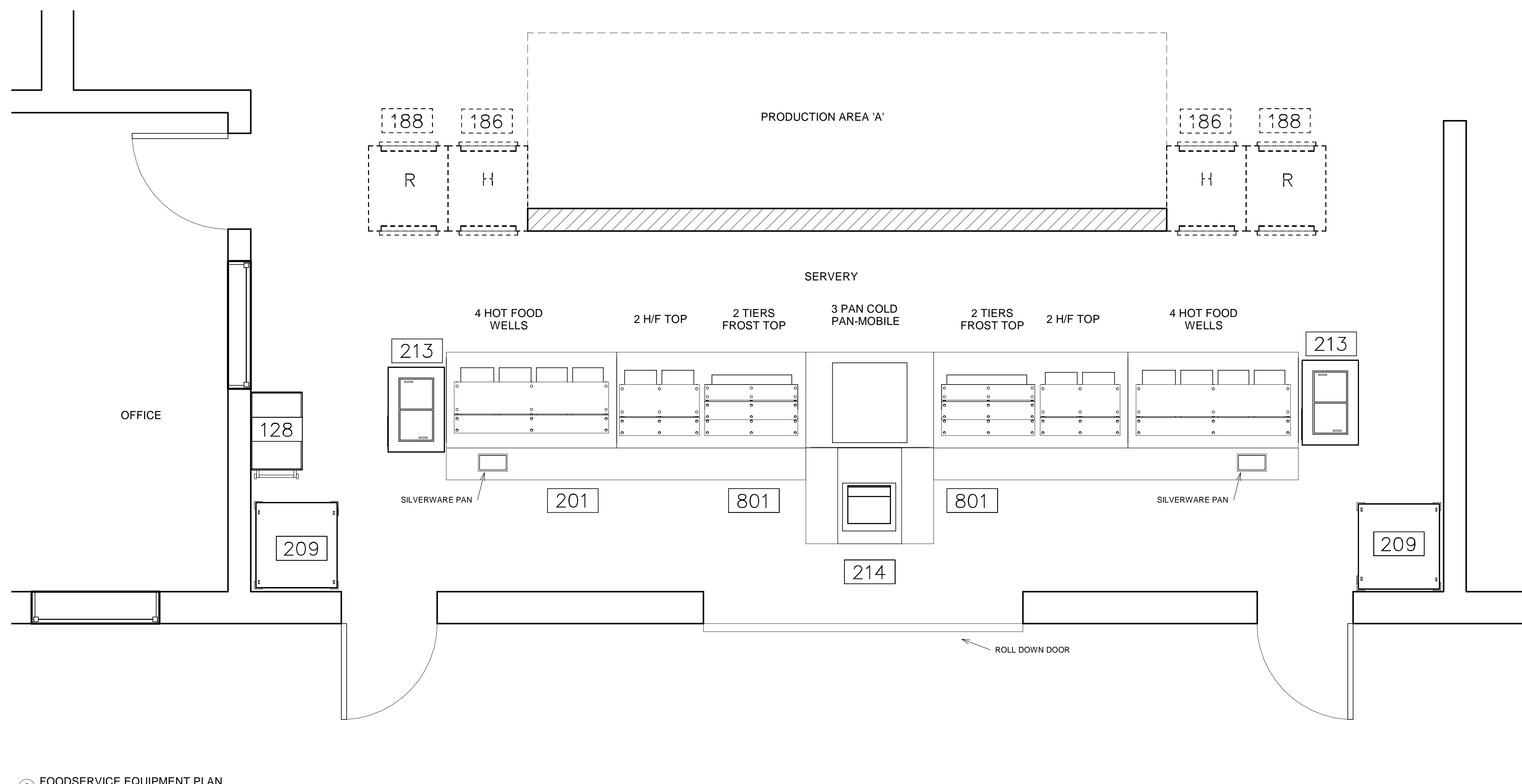
1 FOODSERVICE EQUIPMENT PLAN 1/2" = 1'-0"
