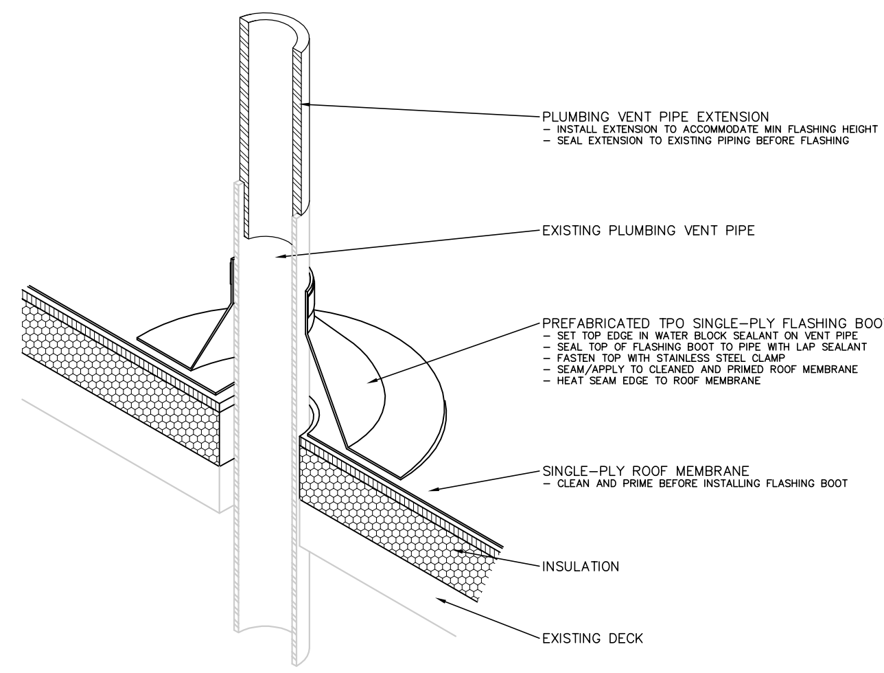
3 PLUMBING VENT WITH EXTENSION N.T.S.
