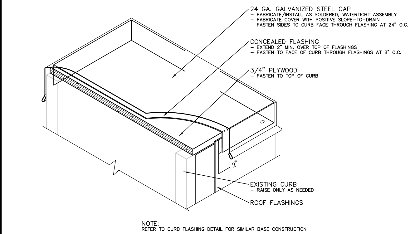
11 ABANDONED CURB FLASHING N.T.S.
