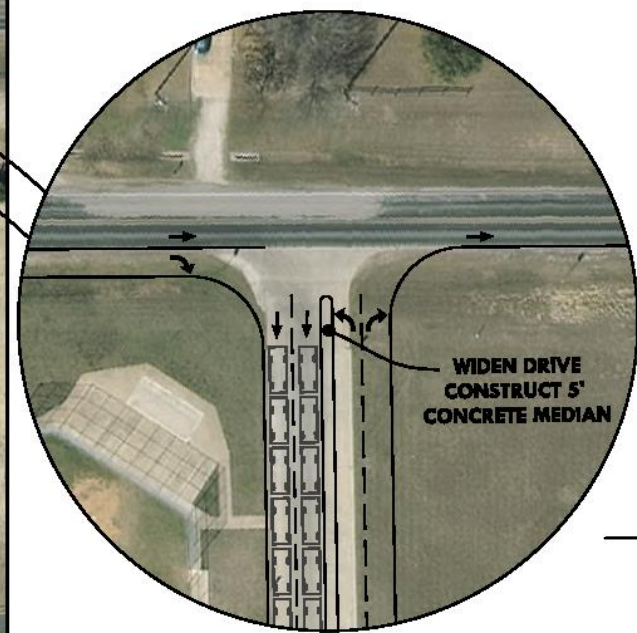
INSET 'A' 1"=80'
