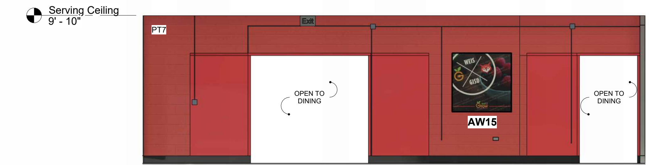
ELEVATION E 1/4" = 1'-0"
