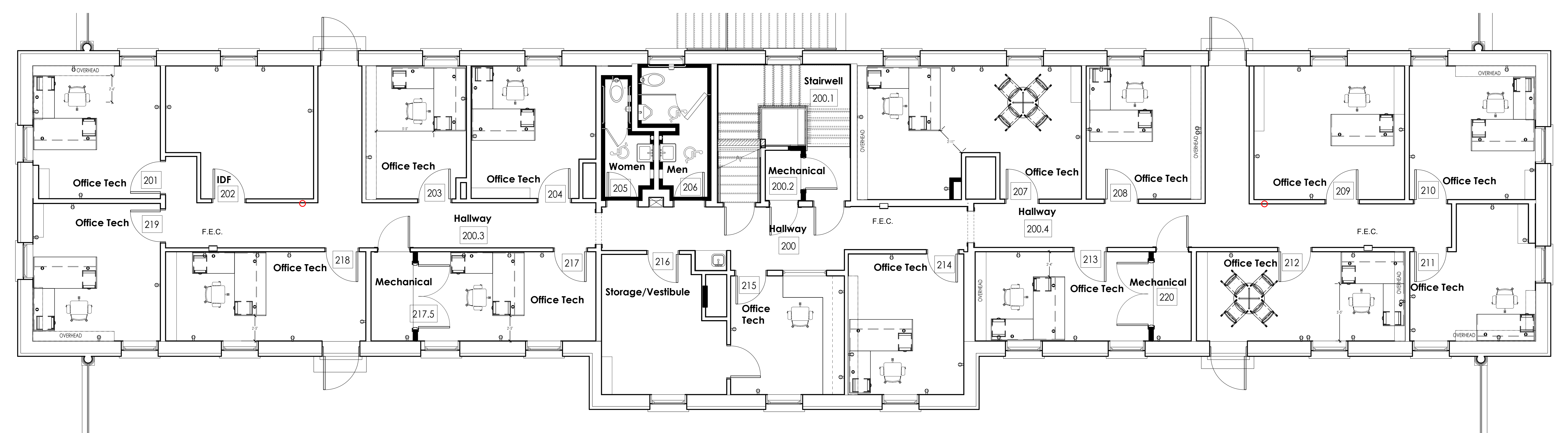
SECOND FLOORPLAN
