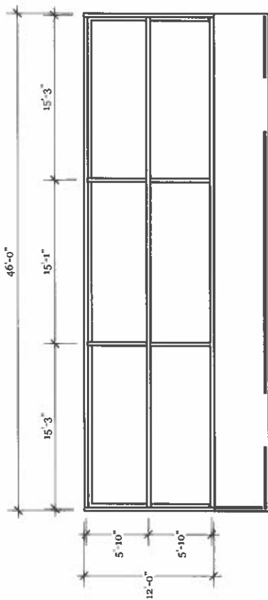
Home Dugout 1/8"=1'-0"
