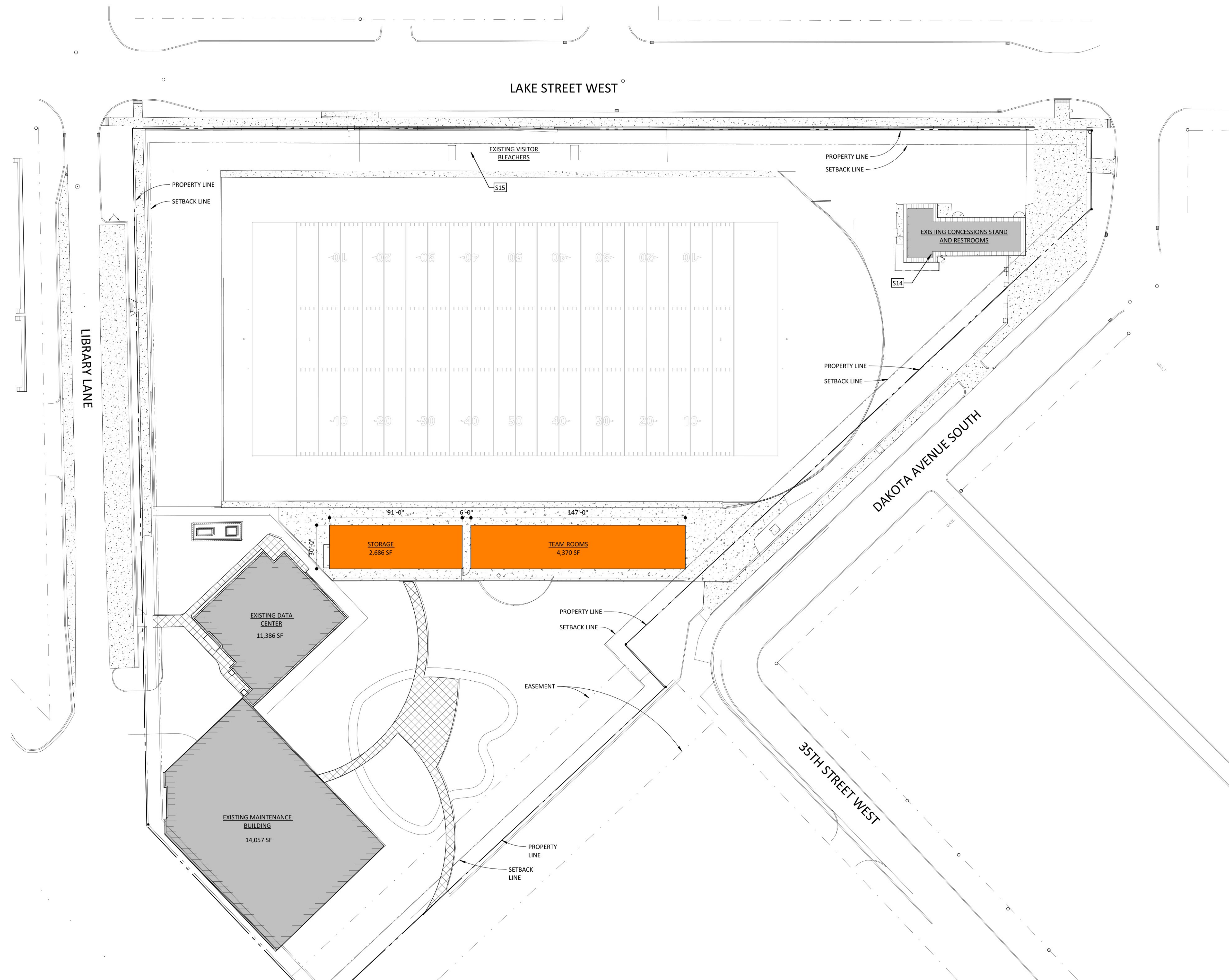
1 ARCHITECTURAL SITE PLAN A1.7 1/32" = 1'-0"
