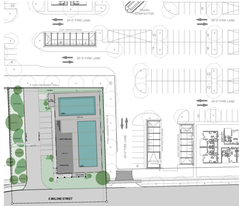
1 CONCEPTUAL SITE PLAN SCALE: 1/4" = 1'-0"
