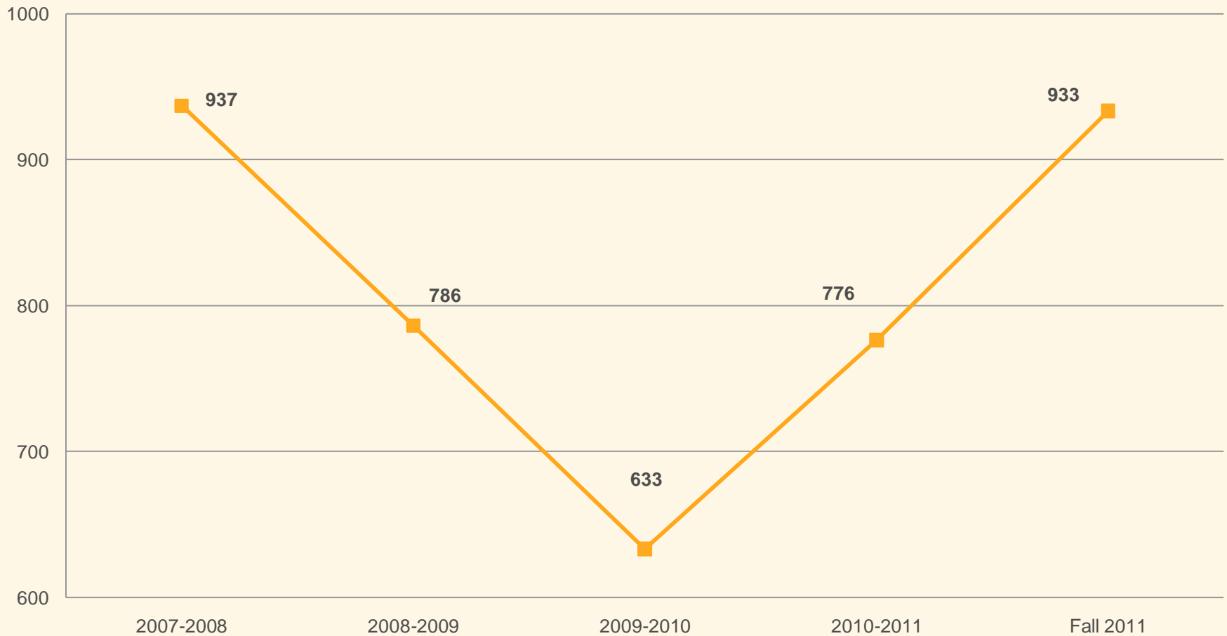
Eligibility Trending
