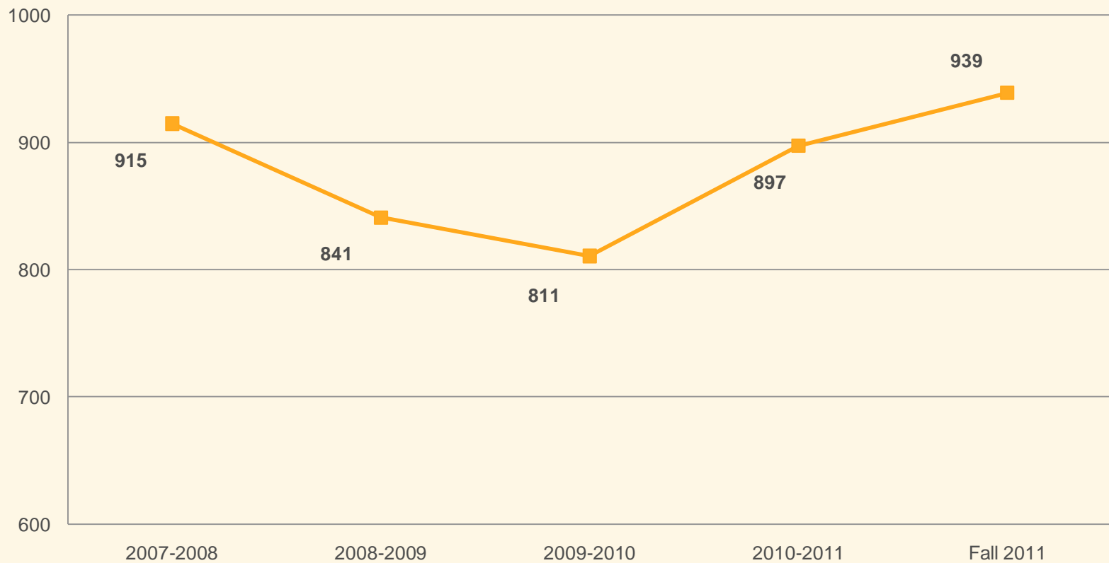
Freshman Trending
