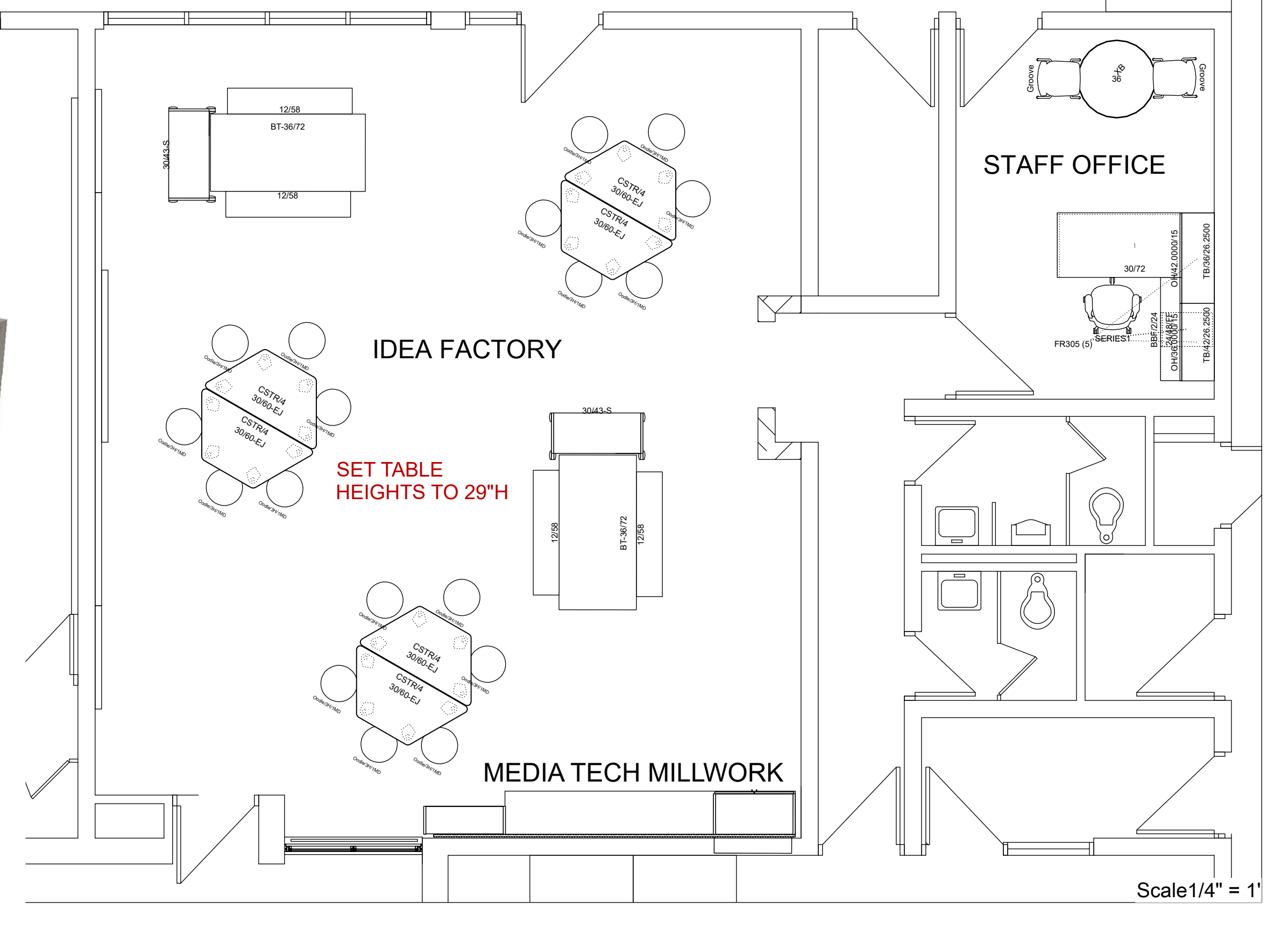
COMPONENT PLAN - MEDIA CENTER
