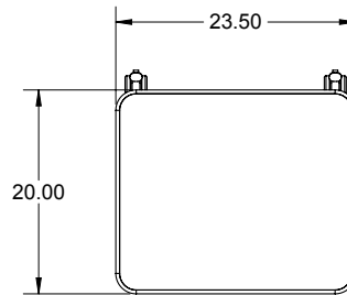
Model 26547v 20"d x 23.5"w Rectangle.
