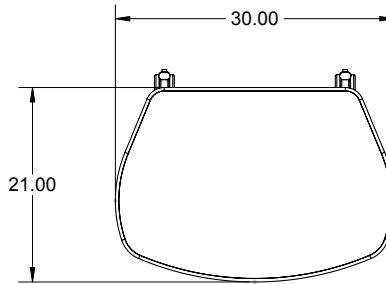
Model 26548 v 21"d x 30"w Collaborative top.
