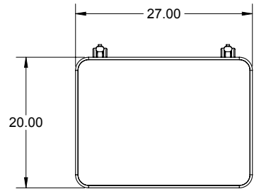
Model 26549 v * 20"d x 27"w Rectangle. * Model 26517 Modesty Panel not compatible with 20x27 desktop.
