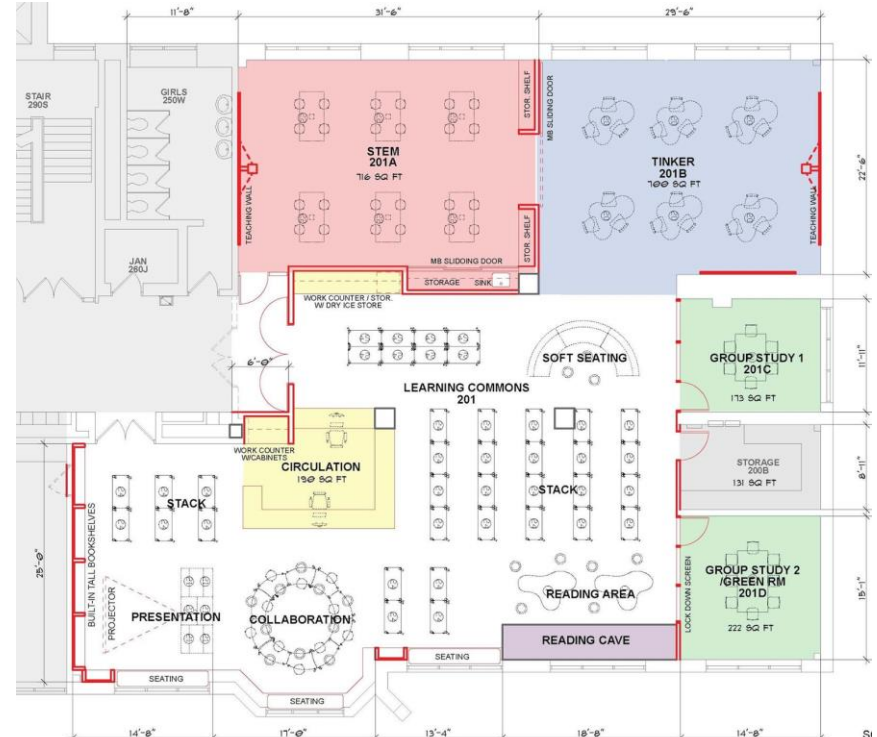
PROPOSED RENOVATION
