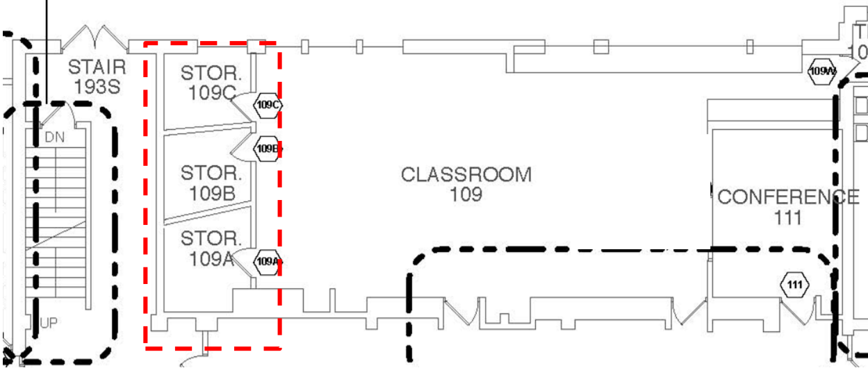
EXISTING LAYOUT
