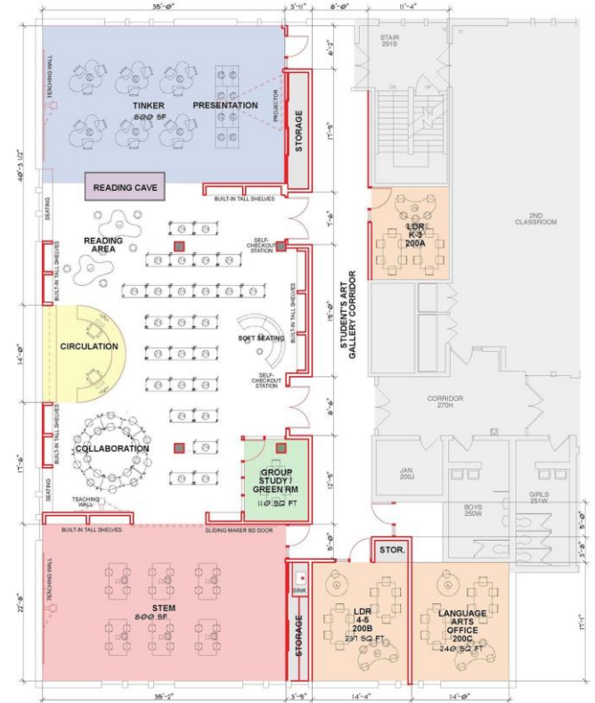
PROPOSED RENOVATION
