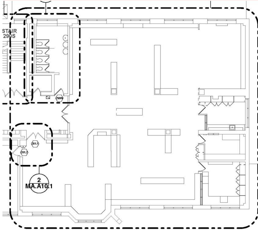
EXISTING LAYOUT
