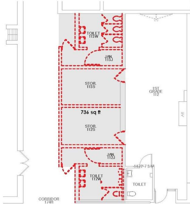
DEMO PLAN
