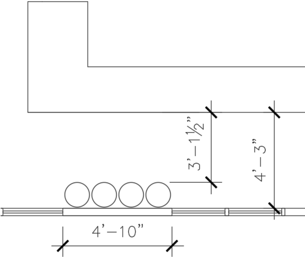
PLAN VIEW
