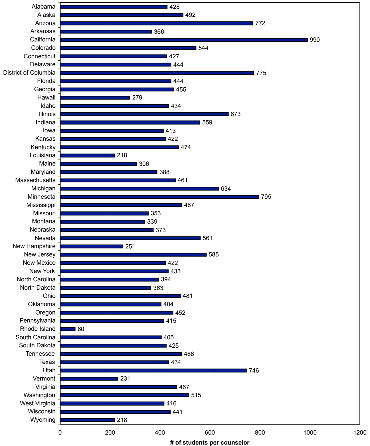
Student-to-School-Counselor Ratio: 2004-2005
