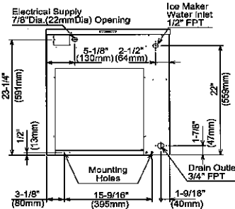
AIR-COOLED UNIT
