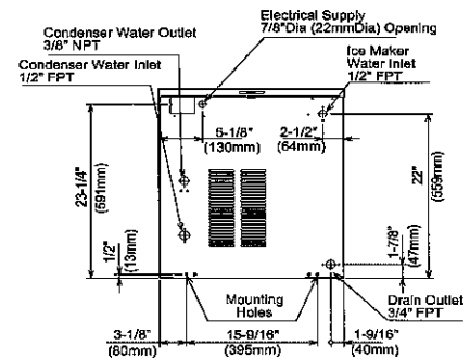
WATER-COOLED UNIT
